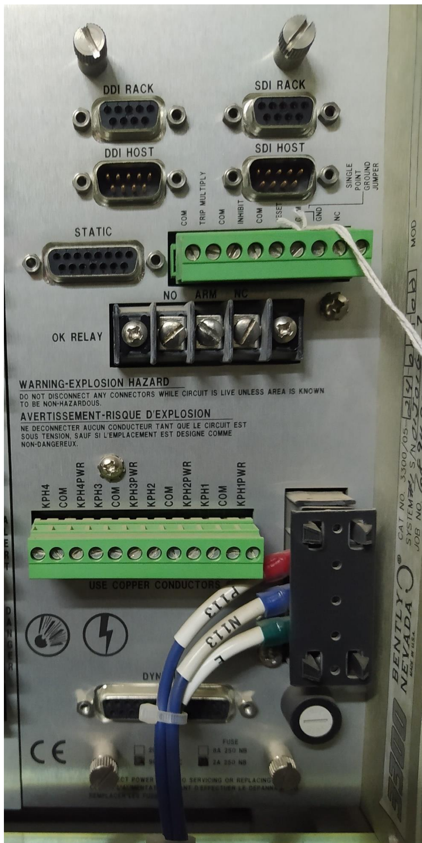
Figure 3: Power Supply for Existing 3300 Rack
