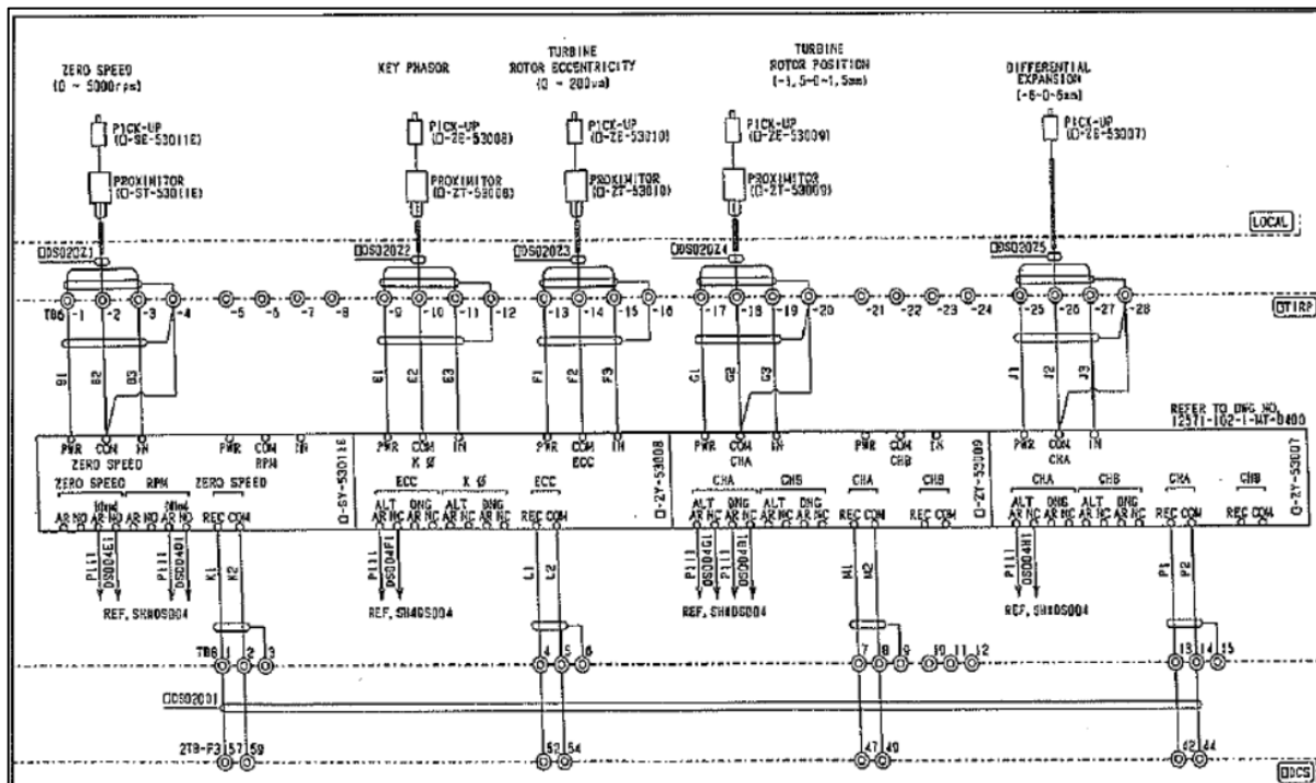
Figure 4: Circuit Diagram for the Existing 3300 Rack System
