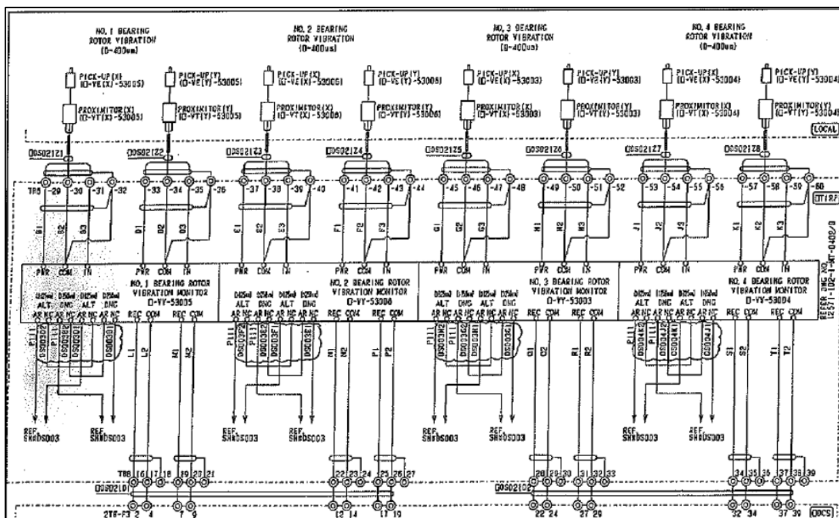
Figure 5: Circuit Diagram #2 for the Existing 3300 Rack System
