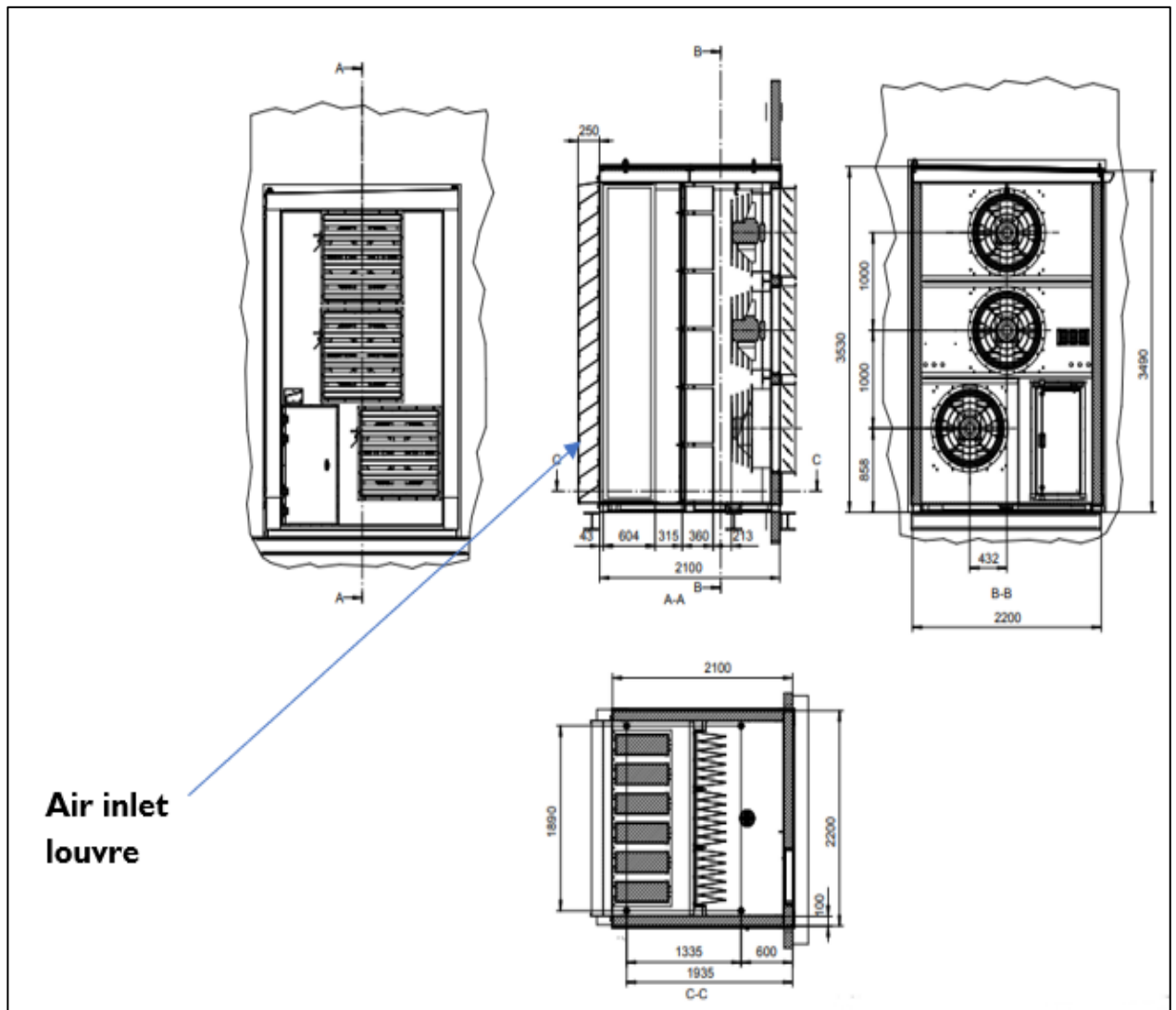
Drawings: Air inlet ventilation filters charge air side
