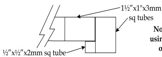
Details of "B" - Door frame
