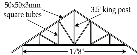
Drawing No. 4 Main truss design
