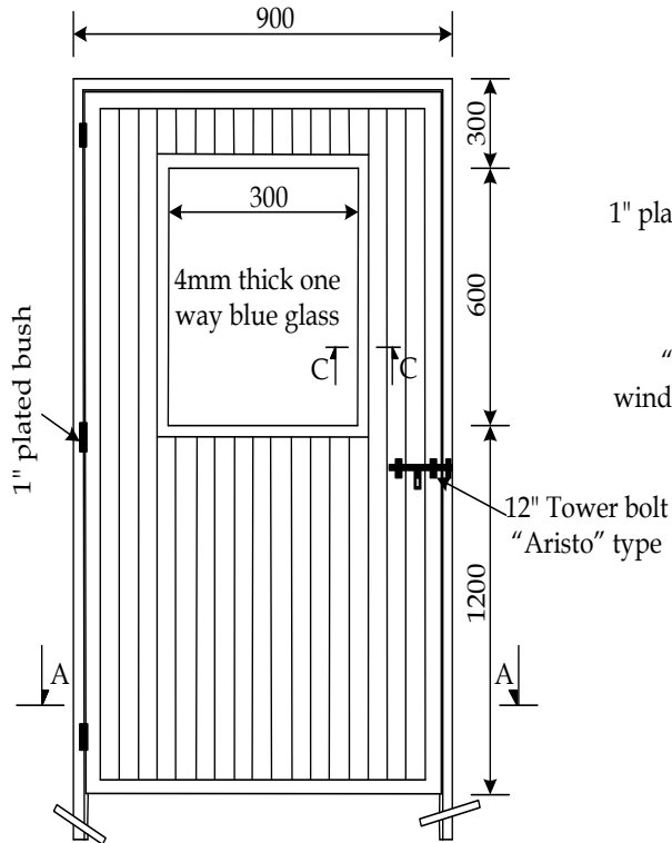
DRAWING NO. 1 CHEMICAL STORE STEEL DOOR
