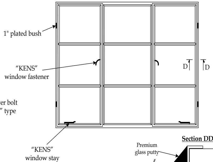
DRAWING NO. 2 CHEMICAL STORE STEEL WINDOW
