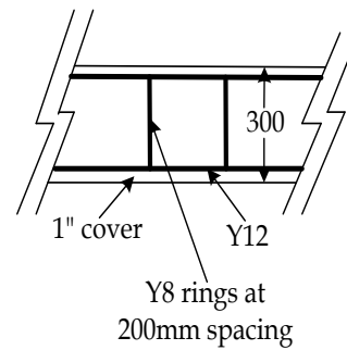
Drawing No. 5 Ring beam design
