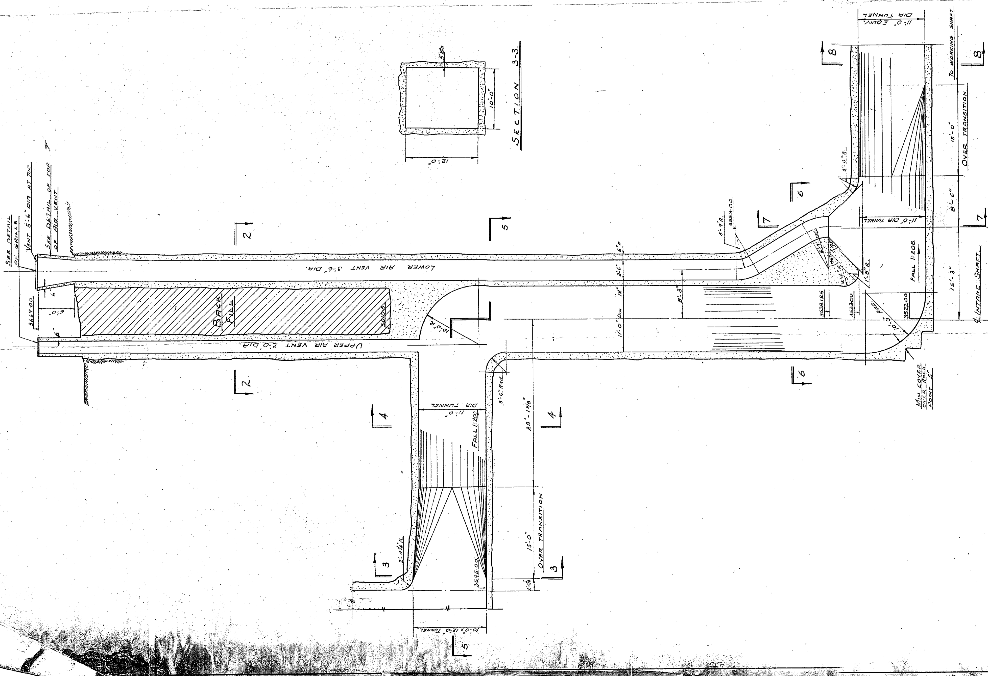
SECTION A-A THROUGH INTAKE SHAFT.
