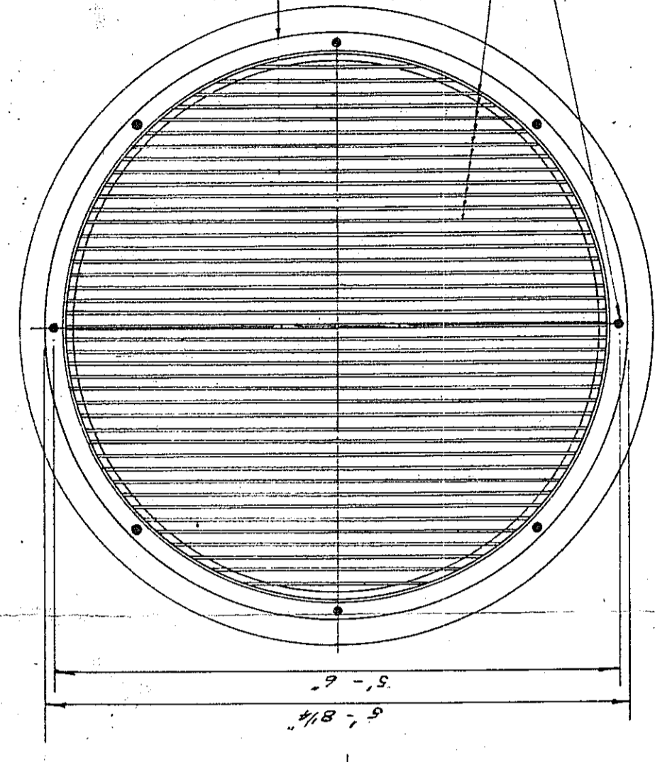
PLAN AT TOP OF LOWER AIR VENT.
