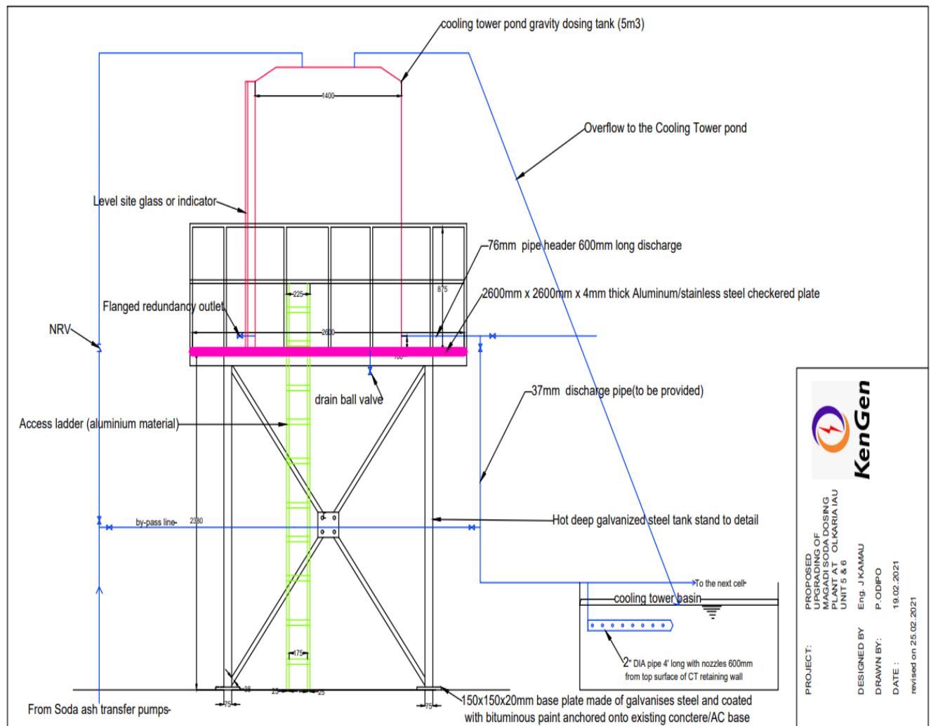
FIG. NO.3: SKETCH DRAWING OF THE GRAVITY DOSING TANK , MOUNTING AND PIPES CONNECTIONS TO IT
