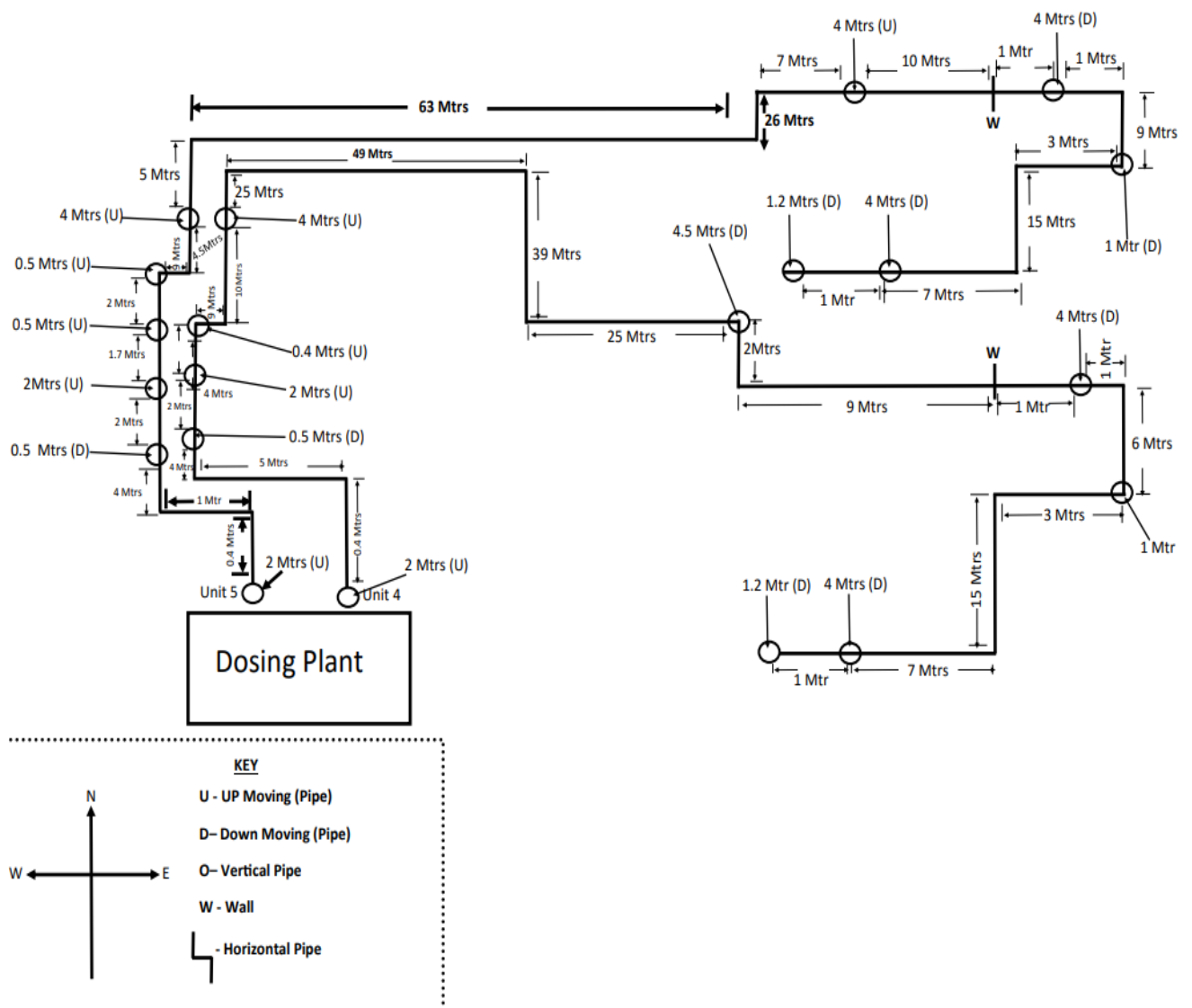
FIG NO. 4: DOSING PIPES LAYOUTS FROM DOSING PUMPS TO RE-INJECTION AND CIRCULATING WATER DOSING POINTS
